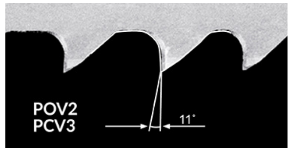
POVII profile in variable tooth pitches 0.8/1.3 & 1.3/2 TPI PCVIII profile in variable tooth pitches 2/3, 3/4, and 4/6
